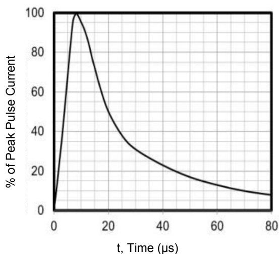
Figure 5. 8 X 20 \mu\text{s} Pulse Waveform
