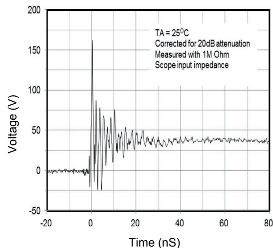
Figure 6. ESD Clamping Voltage 8kV Contact per IEC61000-4-2
