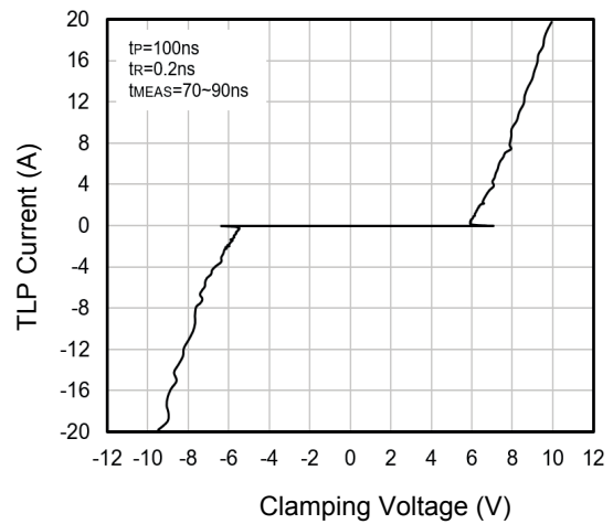
Figure 4. TLP Curve
