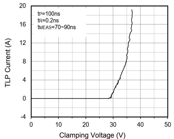
Figure 4. TLP Measurement
