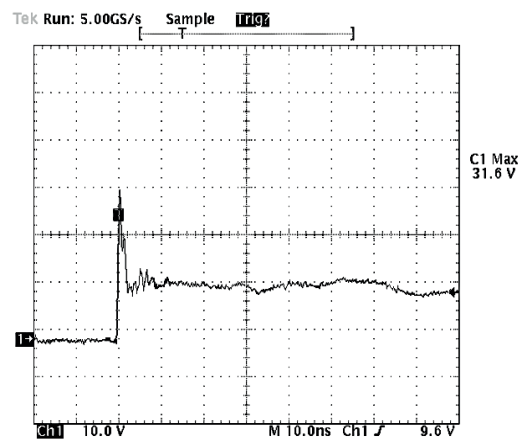
Figure 6. ESD Clamping Voltage
