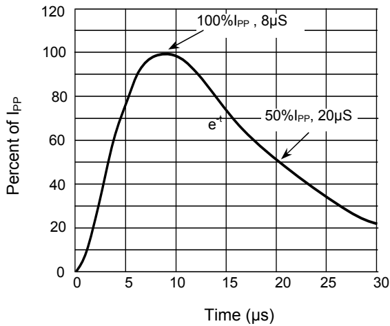
Figure 3. Pulse Waveform-8/20μs
