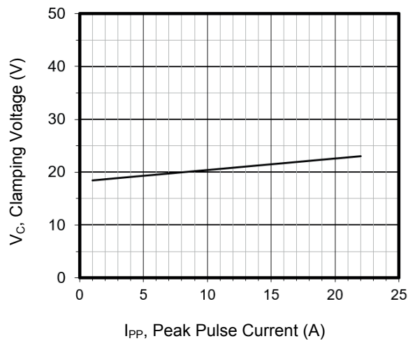
Figure 3. Clamping Voltage vs. Peak Pulse Current ( t_p=8/20\mu\text{s} )
