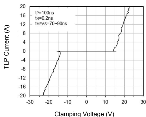
Figure 4. TLP Measurement
