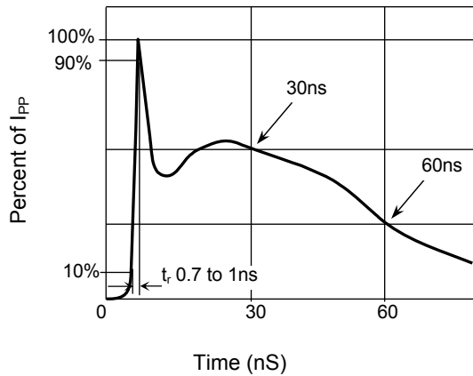
Figure 4. Pulse Waveform-ESD(IEC61000-4-2)
