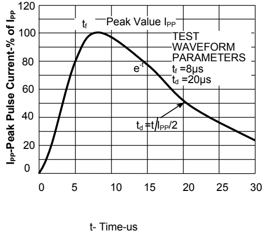
Fig.2 Pulse Waveform
