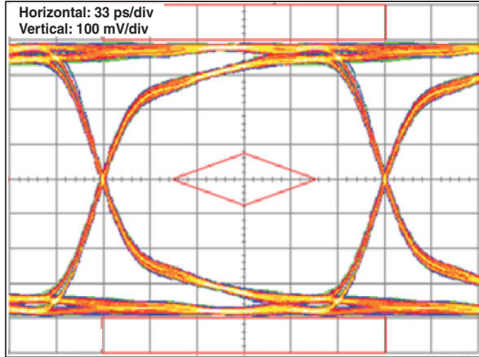
Fig.7 Eye Diagram - USB3.0 mask at 5.0Gbps per channel (with GSESUC5VD0603-2U)
