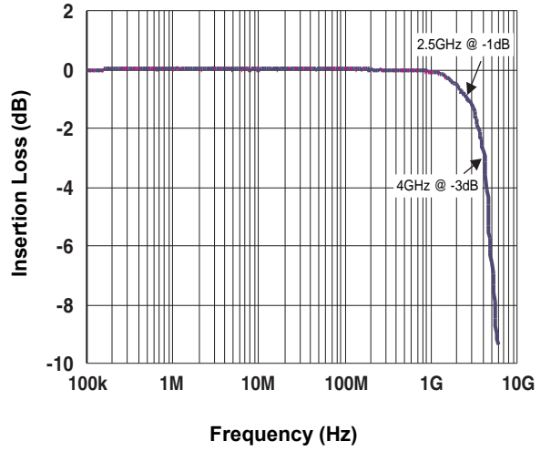
Fig.8 Insertion Loss S21- I/O to GND
