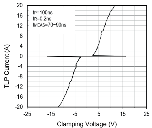
Figure 4. TLP Measurement
