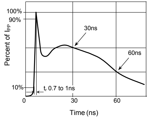
Figure 4. Pulse Waveform-ESD(IEC61000-4-2)
