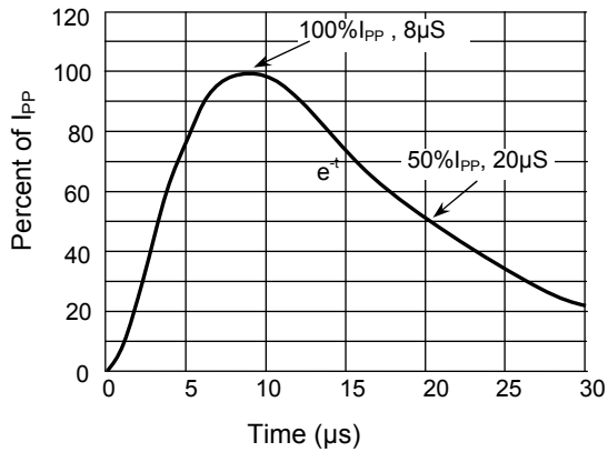
Figure 3. Pulse Waveform-8/20μs
