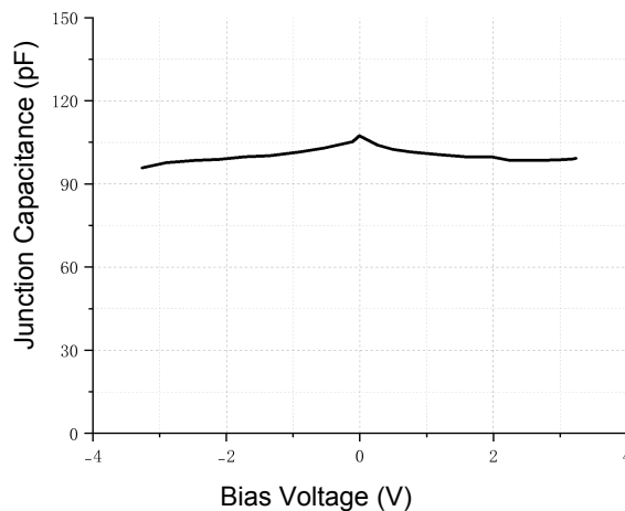
Figure 4. Junction Capacitance Curve
