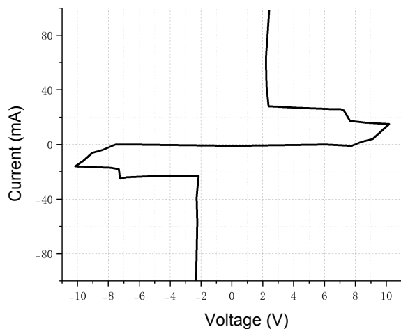
Figure 5. I-V Curve
