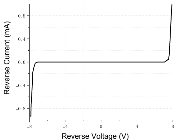
Figure 1. Breaking Voltage Curve
