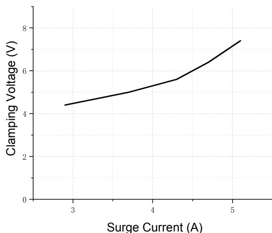
Figure 3. 8/20 \mu s Surge Current Curve
