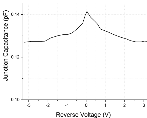
Figure 4. Junction Capacitance Curve
