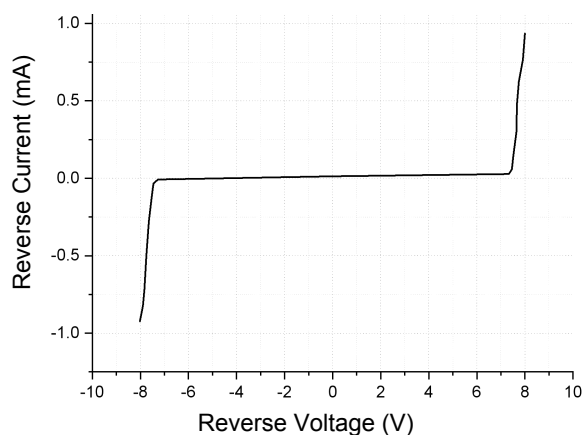
Figure 1. Breaking Voltage Curve
