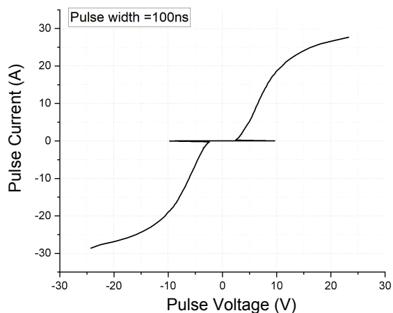
Figure 5. TLP Curve
