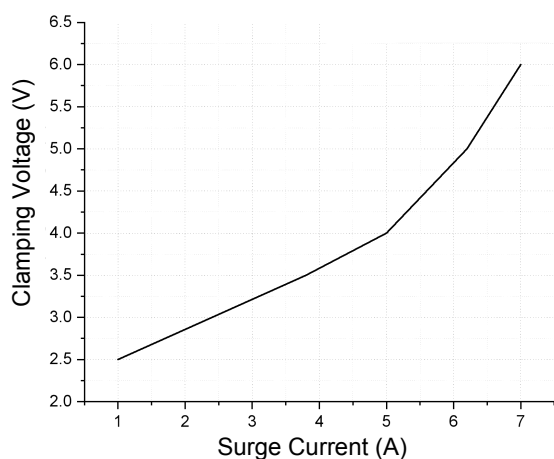
Figure 3. 8/20 \mu s Surge Curve
