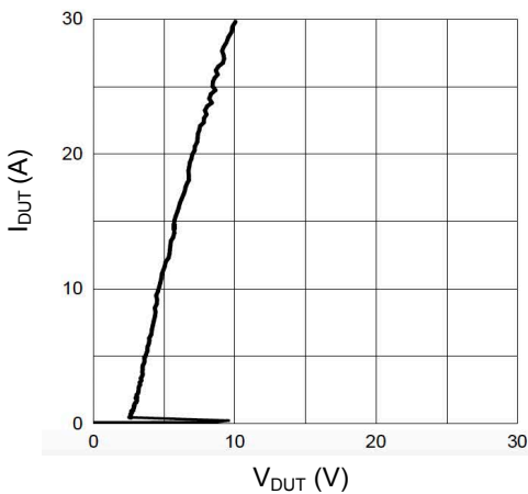
Figure 5. Transmission Line Pulse ( T_p=100ns )
