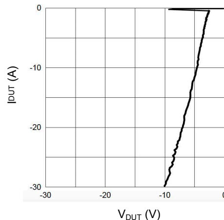
Figure 6. Transmission Line Pulse ( T_p=100ns )
