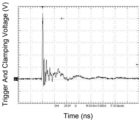
Figure 3. IEC61000-4-2 +8kV Contact Discharge
