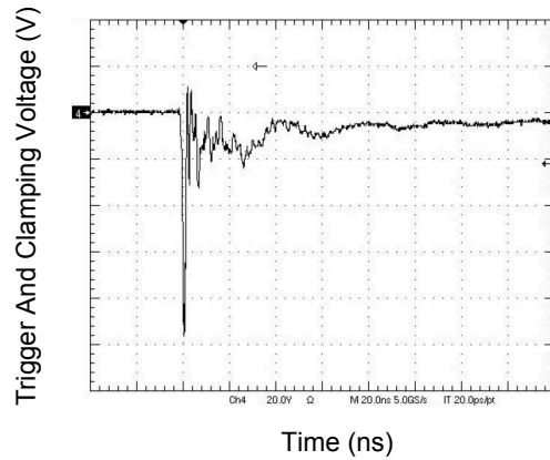
Figure 4. IEC61000-4-2 -8kV Contact Discharge
