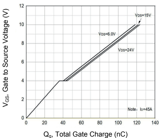
Figure 6. Gate Charge
