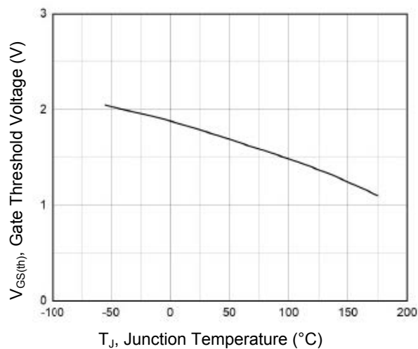
Figure 9. Gate Threshold Voltage vs. T_J
