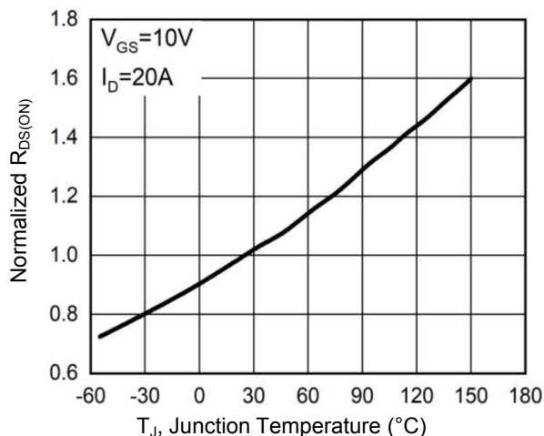
Figure 3. Normalized R_{DS(on)} vs. T_J
