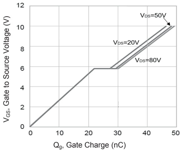
Figure 3. Gate Charge
