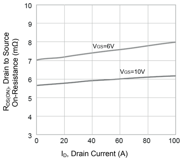
Figure 5. R_{DS(ON)} vs. Drain Current
