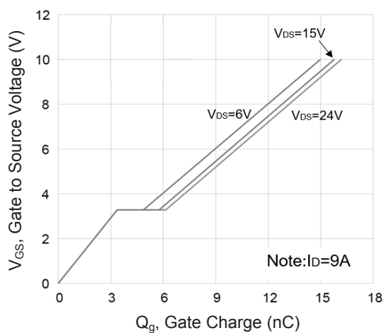
Figure 6. Gate Charge
