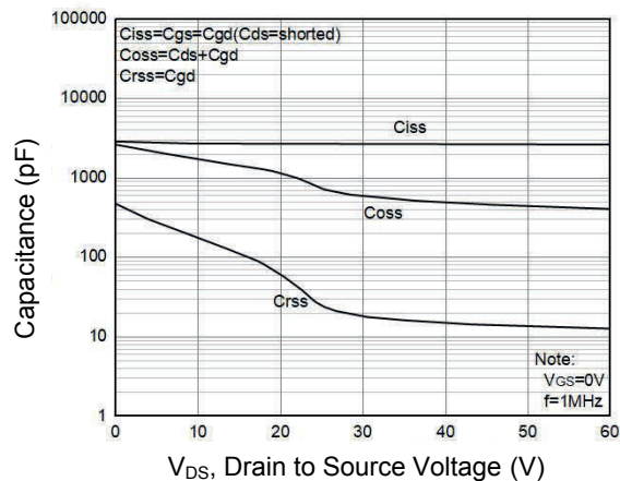
Figure 7. Capacitance Characteristics
