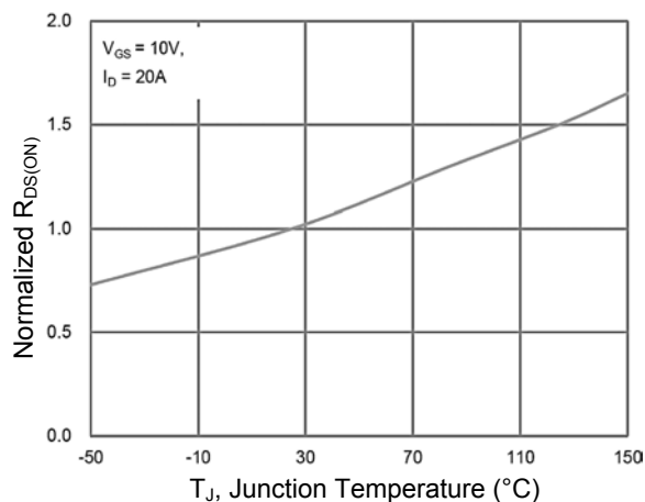
Figure 7. Normalized R_{DS(ON)} vs. T_J
