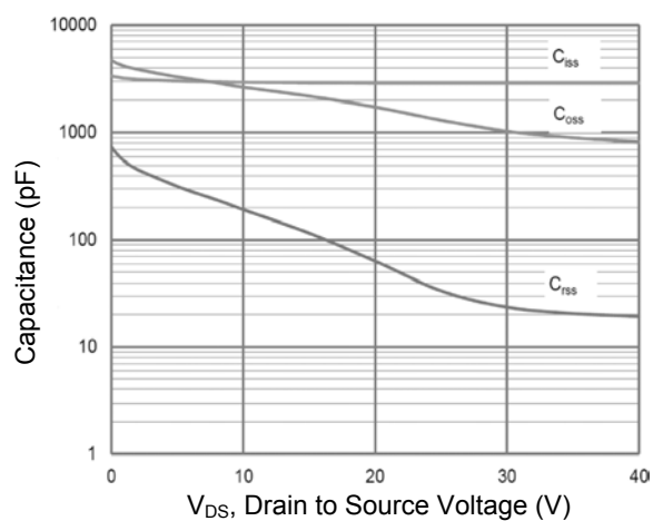
Figure 9. Capacitance Characteristics
