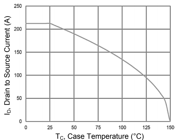
Figure 8. Current Derating
