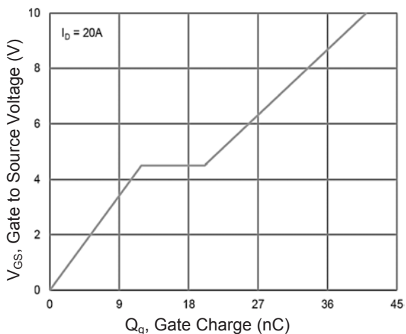
Figure 6. Gate Charge
