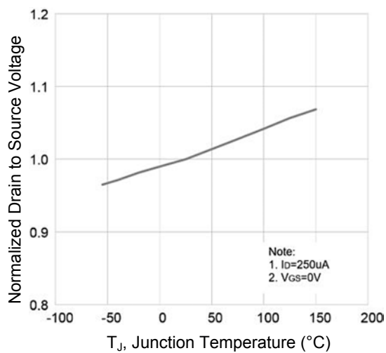
Figure 6. Normalized BV_{DSS} vs. T_J
