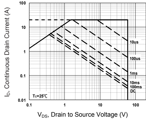
Figure 8. Maximum Safe Operation Area
