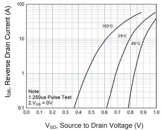
Figure 4. V_{SD} vs. I_{DR}
