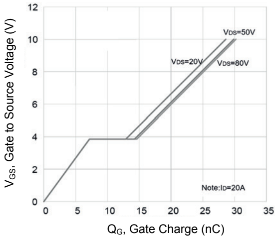
Figure 3. Gate Charge
