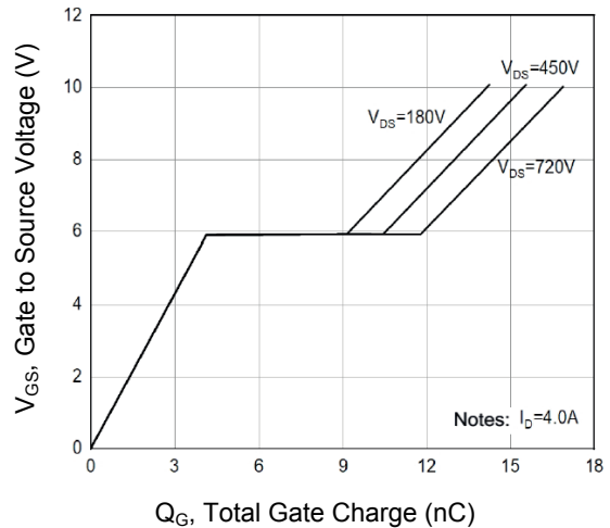
Figure 6. Gate Charge
